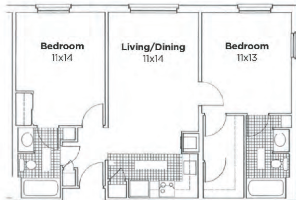
Two Bedroom Floor Plan
